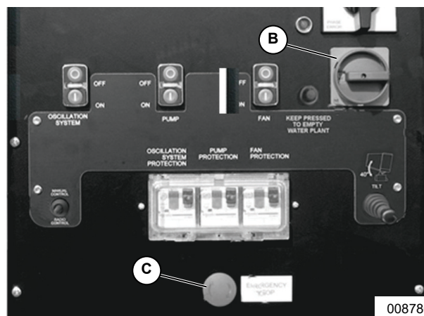
Figure 2-8. Emergency Stop Button
