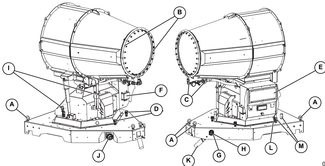
Figure 2-2. Component Locations
