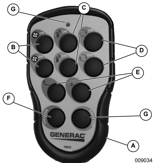
Figure 3-9. Transmitter
