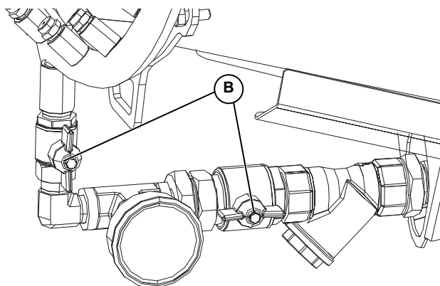
Figure 3-2. Water Control Valves
