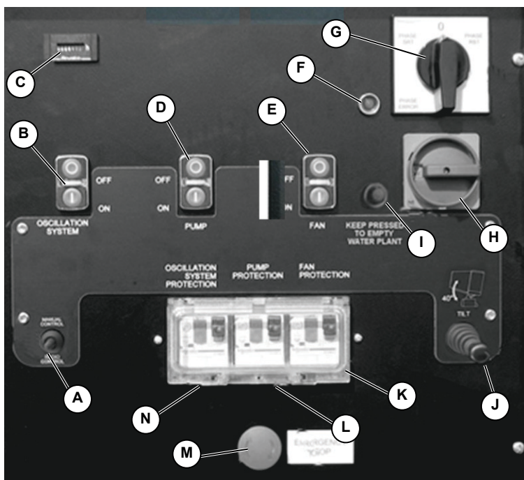
Figure 2-4. Control Panel
