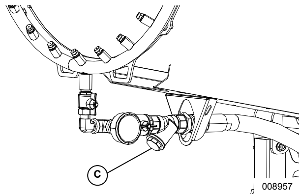
Figure 4-5. Nozzle Water Filters
