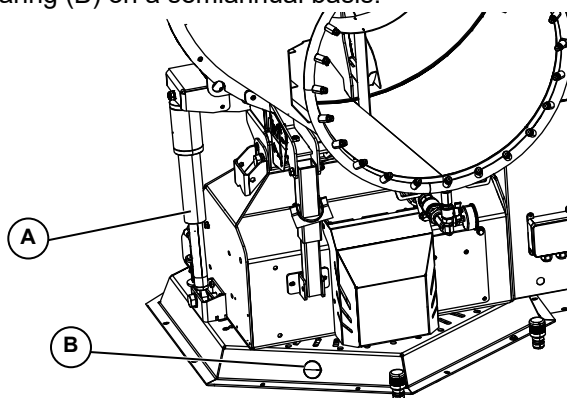
Figure 4-7. Lubrication
