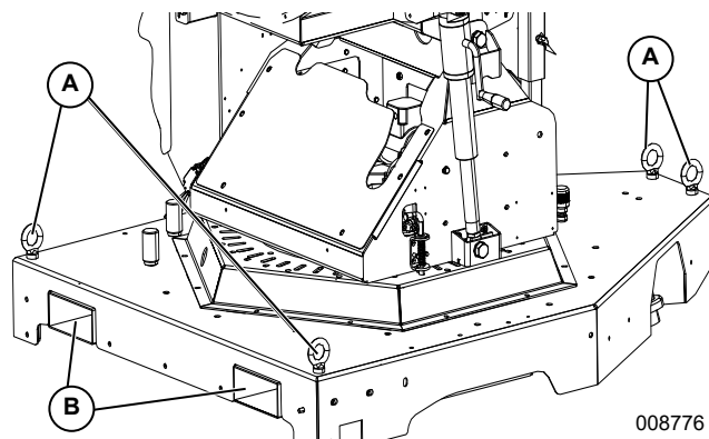
Figure 2-11. Lifting Points
