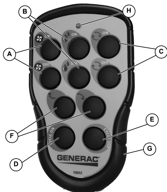
Figure 2-4. Transmitter Unit
