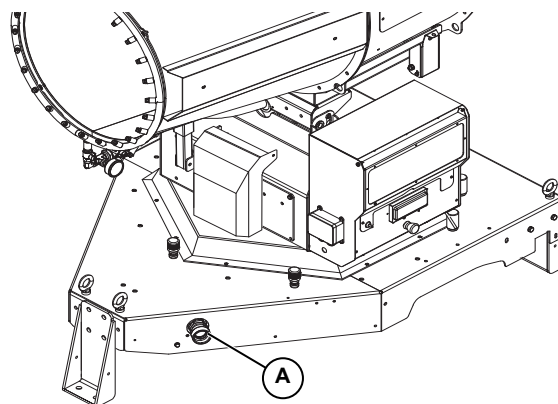
Figure 3-1. Water Connection
