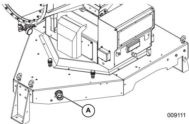
Figure 2-6. Water Connection
