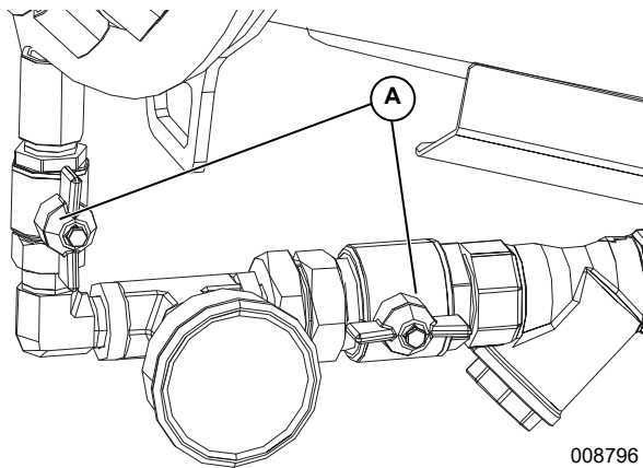
Figure 4-2. Open Valves
